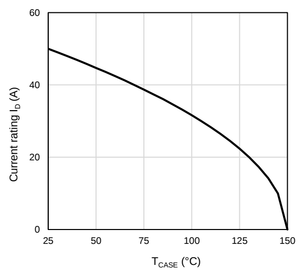
Figure 12: Current De-rating
