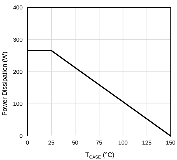
Figure 11: Power De-rating
